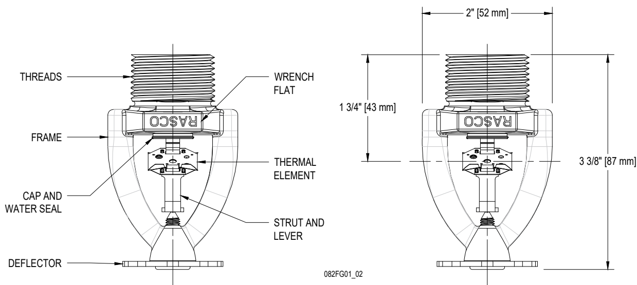
Model N28T3 Sprinkler Components and Dimensions
