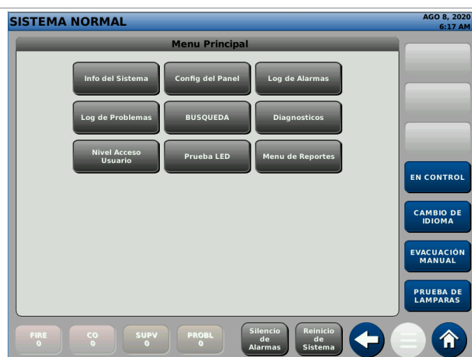
Figura 4: Menú Principal
